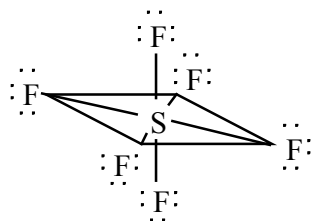
11. \text{SF}_6 octahedral
