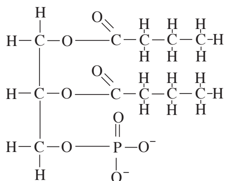
Fig. 18 Phosphatidic acid.
