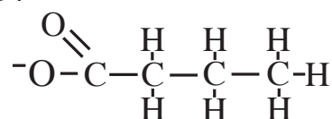
Fig. 19 A soap.
