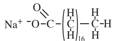
Fig. 9 Soap.
