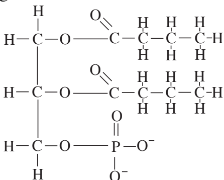
Fig. 7 Phosphatidic acid.
