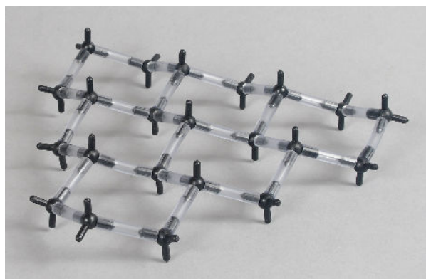
Fig. 3 Six hexagons.
