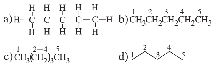
Fig.1 Four methods of drawing pentane.
